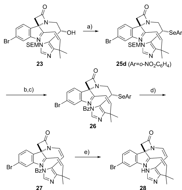
Scheme 9. a) o -NO 2 C 6 H 4 SeCN, n Bu 3 P, THF, RT, 62%; b) TfOH, CH 2 Cl 2 , –78 to 0°C; c) BzCl, Et 3 N, DMAP, CH 2 Cl 2 /THF (2:1), RT, 72% (2 steps); d) m CPBA, CH 2 Cl 2 , RT, 80%; e) Na 2 CO 3 , THF/H 2 O (2:1), RT, 63%. Bz = benzoyl, DMAP = 4-(dimethylamino)pyridine, m CPBA = m -chloroperbenzoic acid.
